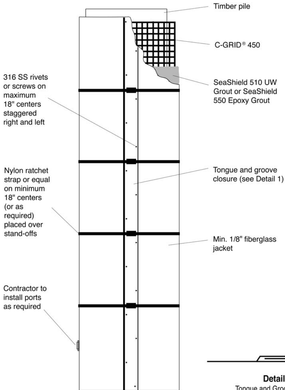
Elevation View
