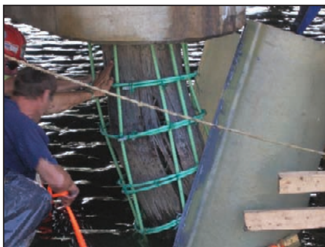
Rebar cage being fixed to the badly damaged pile.
