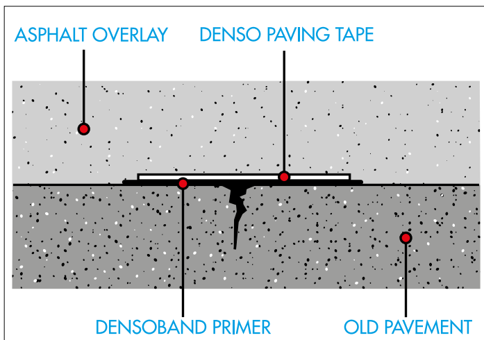
RE-INSTATEMENT TAPE
