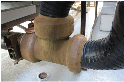
Piping protected with an HDPE Outerwrap and Smartband Strapping system.
