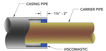
Fig. 2: Pack ViscoMastic a minimum of 1½" - 2" into void.
