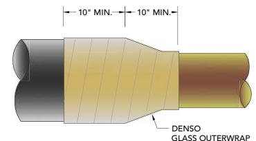
Fig. 5: Apply Denso Glass Outerwrap over ViscoWrap layer. Start wrapping min. 10" from casing end and continue \geq 10" on carrier pipe.
